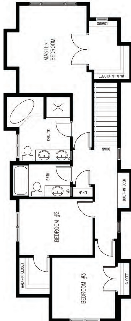
Upper Level 921 sq.ft.
